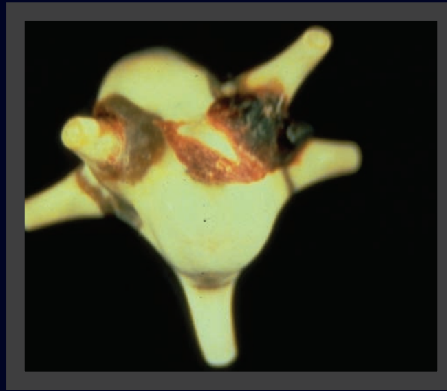
Calcium oxalate dihydrate/calcium oxalate monohydrate
