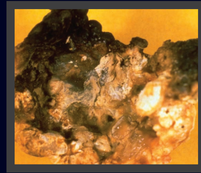
Uric acid/calcium oxalate monohydrate
